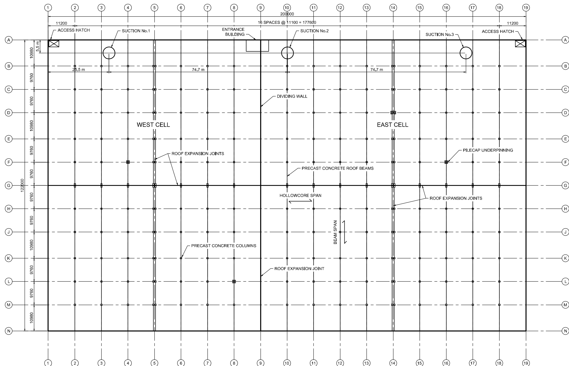
GRIDLINE LOCATION PLAN 1:350
